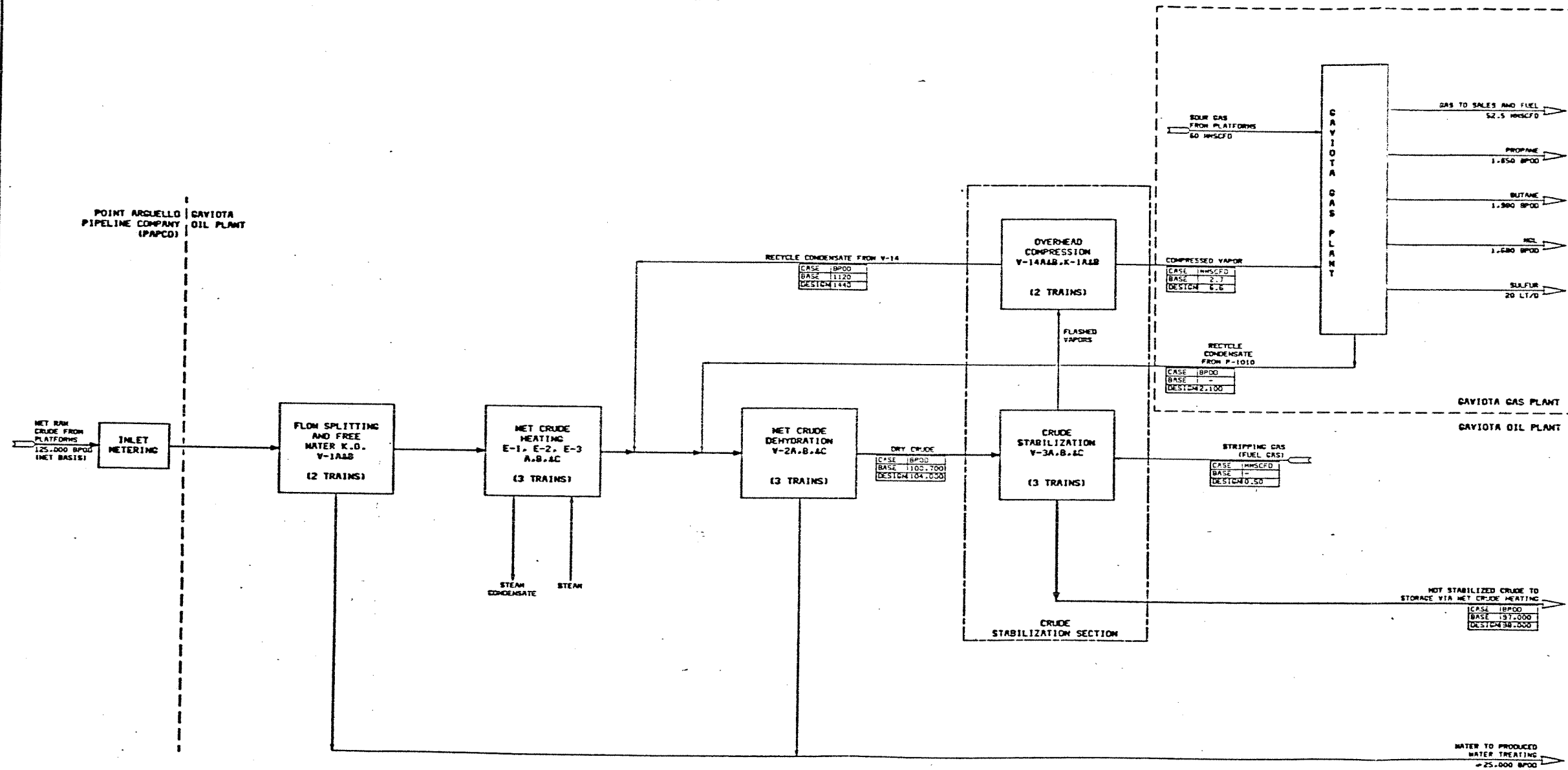
Figure 1.3 Overall Block Flow Diagram Gaviota Oil Plant
